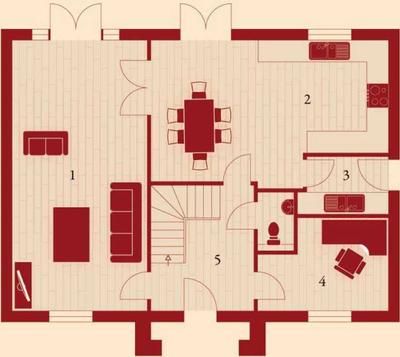
GROUND FLOOR 1. Living 2. Kitchen / Family 3. Utility 4. Study 5. Entrance Hall
